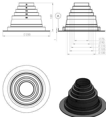
Roofseal no.2
