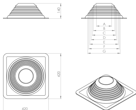
Roofseal no.5
