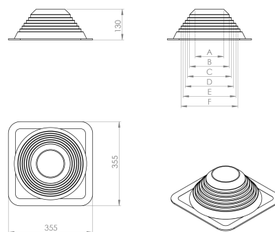
Roofseal no.4
