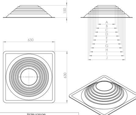
Roofseal no.6
