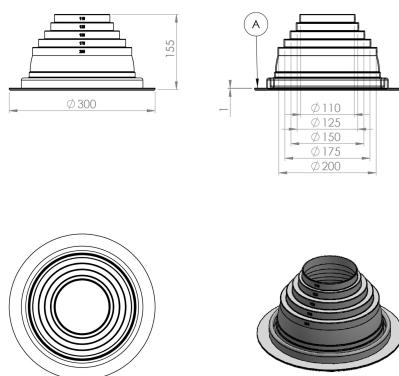
Roofseal no.3
