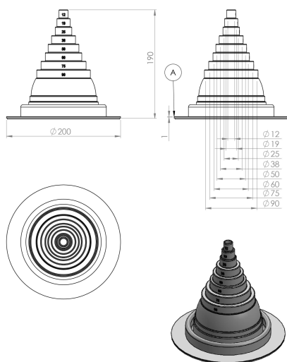
Roofseal no.1
